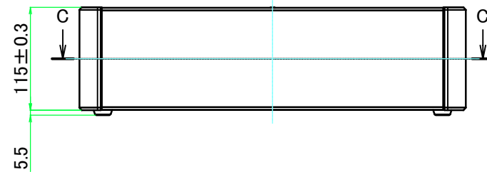
A view
