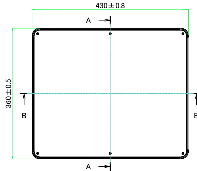
E view
